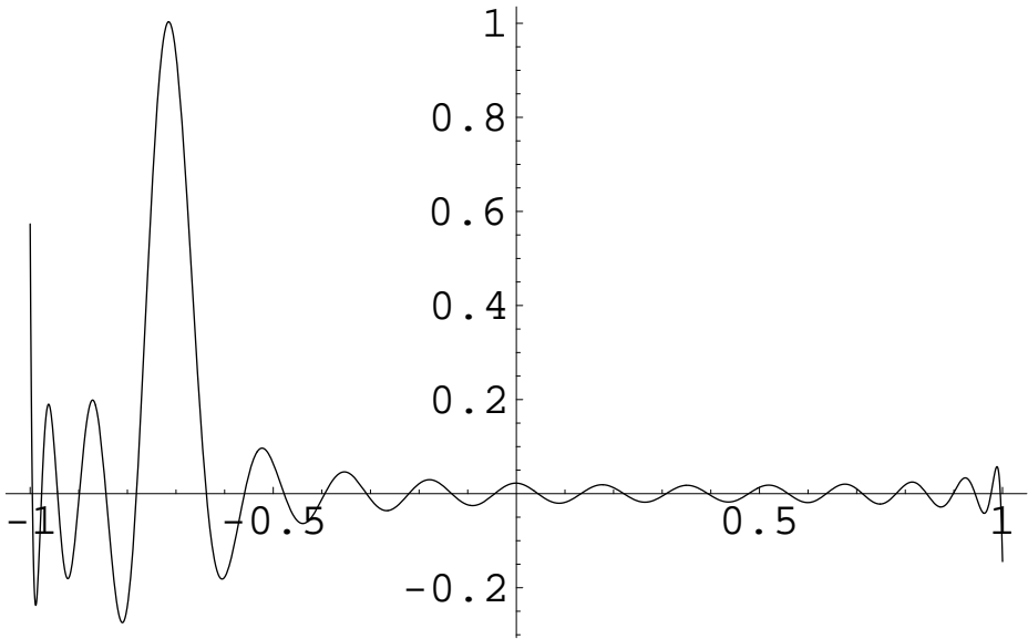
Figure 10: Interpolating function R_7(t) on the interval [-1, 1] .
