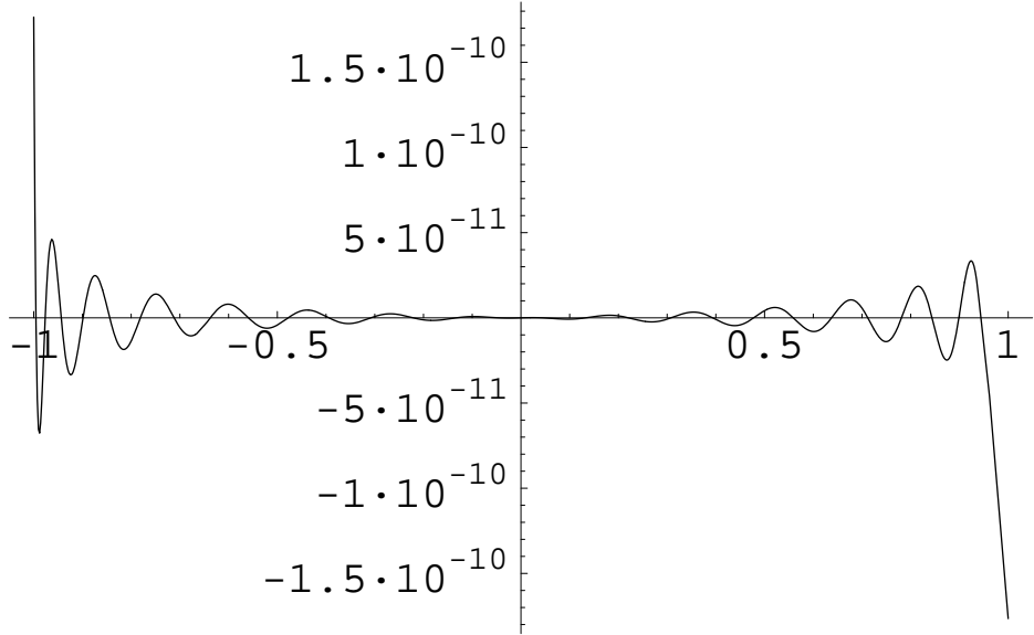
Figure 14: Difference g_2(t) - \tilde{g}_2(t) on the interval [-1, 1] .
