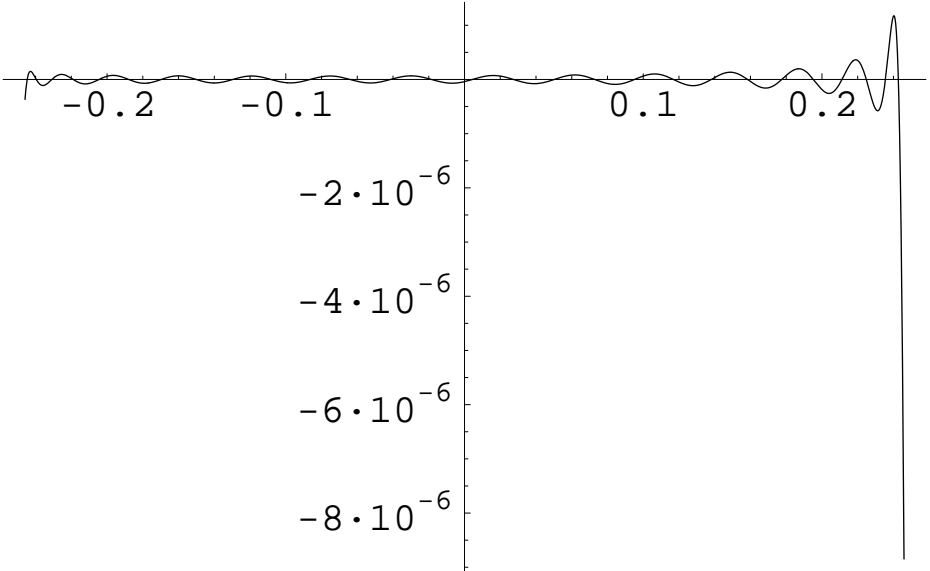
Figure 8: The same function of Figure 7 on the interval [-1/4, 1/4] .
