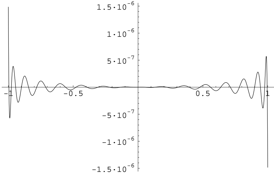
Figure 16: Difference g_3(t) - \tilde{g}_3(t) on the interval [-1, 1] .
