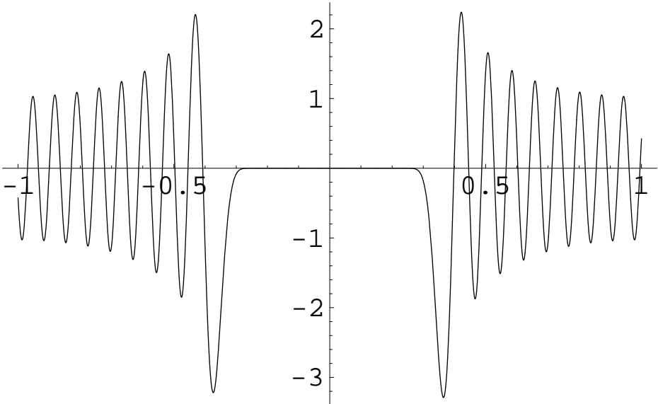
Figure 7: Modified eigenpolynomial (see Figure 2) on the interval [-1, 1] corresponding to the eigenvalue \lambda^{(28)} in Example 3.
