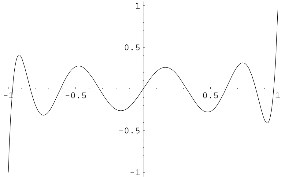
Figure 15: Function g_3(t) on the interval [-1, 1] .
