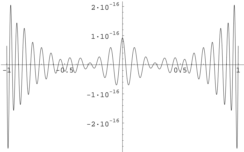
Figure 9: Error in (8.1) for Example 1.
