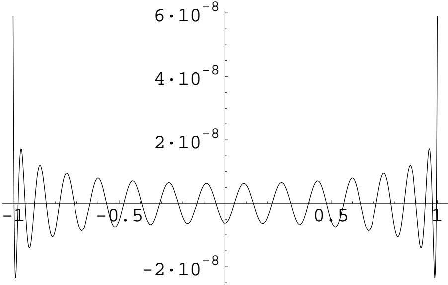
Figure 12: Difference g_1(t) - \tilde{g}_1(t) on the interval [-1, 1] .
