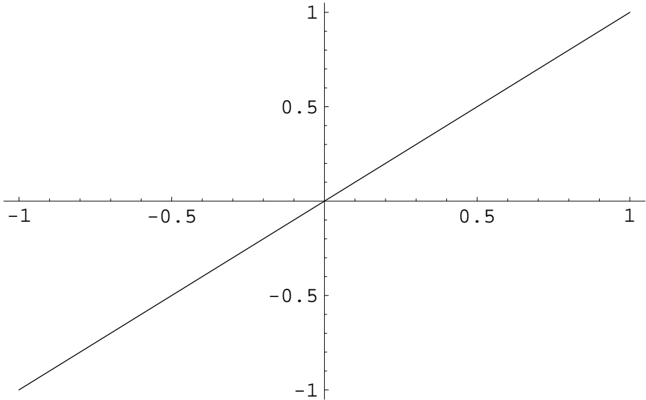
Figure 13: Function g_2(t) on the interval [-1, 1] .
