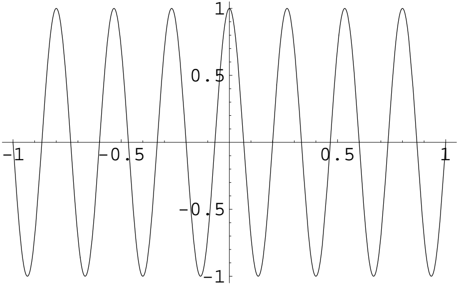
Figure 11: Function g_1(t) on the interval [-1, 1] .
