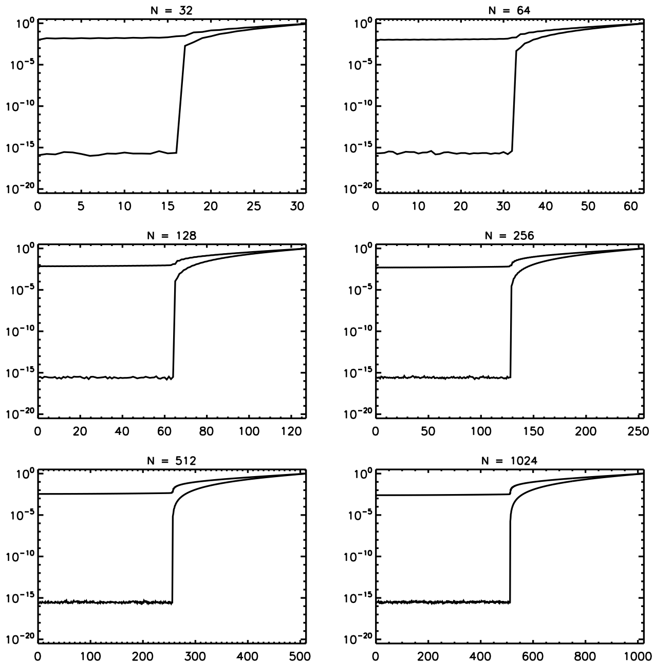
Fig. 2. Plots of \mathcal{E}_{j,N/2}^{(1)} and \mathcal{E}_{j,N/2}^{(2)} for the sine transform of a cosine function for N \in \{32, 64, 128, 256, 512, 1024\} and j \leq N . In each plot, the top line shows \mathcal{E}_{j,N/2}^{(1)} and the bottom line shows \mathcal{E}_{j,N/2}^{(2)} . For clarity, the ratios, \mathcal{E}_{j,N/2}^{(2,1)} , are not shown.
