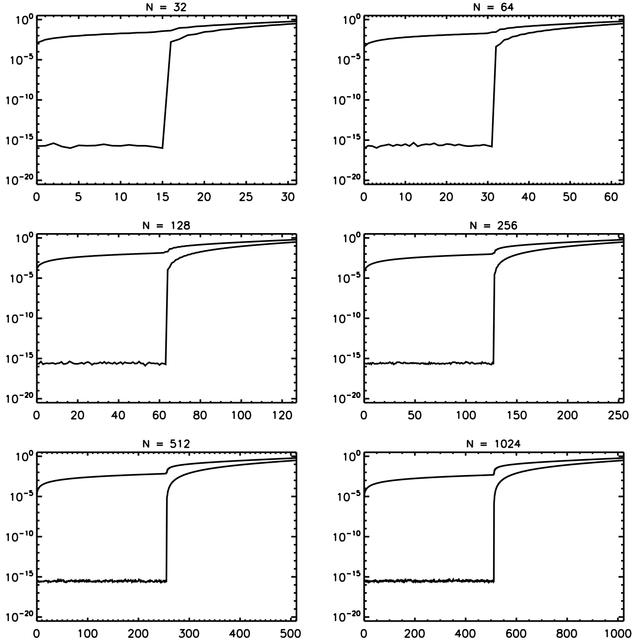
Fig. 5. Plots of \mathcal{E}_{j,N/2}^{(1)} and \mathcal{E}_{j,N/2}^{(2)} for the cosine transform of a sine function for N \in \{32, 64, 128, 256, 512, 1024\} and j \leq N . In each plot, the top line shows \mathcal{E}_{j,N/2}^{(1)} and the bottom line shows \mathcal{E}_{j,N/2}^{(2)} . For clarity, the ratios, \mathcal{E}_{j,N/2}^{(2,1)} , are not shown.
