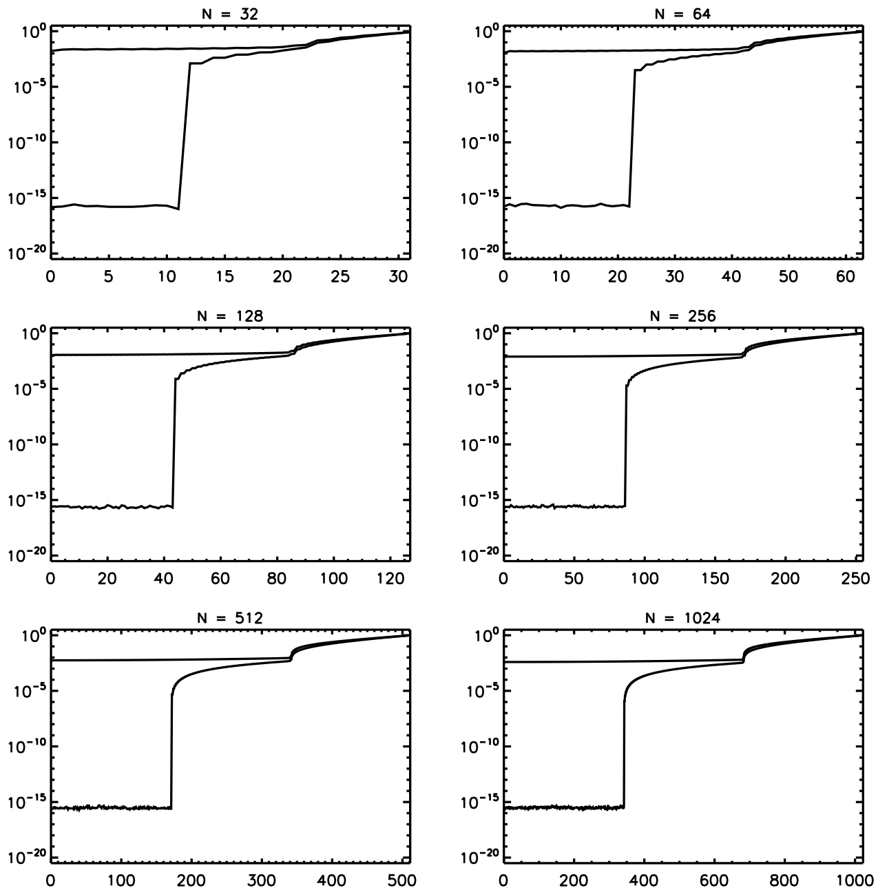
Fig. 3. Plots of \mathcal{E}_{j, \lfloor 2N/3 \rfloor}^{(1)} , and \mathcal{E}_{j, \lfloor 2N/3 \rfloor}^{(2)} for the sine transform of a cosine function for N \in \{32, 64, 128, 256, 512, 1024\} and j \leq N . In each plot, the top line shows \mathcal{E}_{j, \lfloor 2N/3 \rfloor}^{(1)} and the bottom line shows \mathcal{E}_{j, \lfloor 2N/3 \rfloor}^{(2)} . For clarity, the ratios, \mathcal{E}_{j, \lfloor 2N/3 \rfloor}^{(2,1)} , are not shown.
