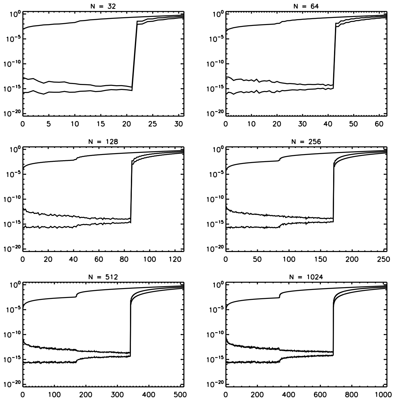
Fig. 4. Plots of \mathcal{E}_{j,[N/3]}^{(1)} , \mathcal{E}_{j,[N/3]}^{(2)} , and \mathcal{E}_{j,[N/3]}^{(2,1)} for the cosine transform of a sine function for N \in \{32, 64, 128, 256, 512, 1024\} and j \leq N . In each plot, the top line shows \mathcal{E}_{j,[N/3]}^{(1)} , the bottom line shows \mathcal{E}_{j,[N/3]}^{(2)} and the intermediate line shows the ratios, \mathcal{E}_{j,[N/3]}^{(2,1)} .
