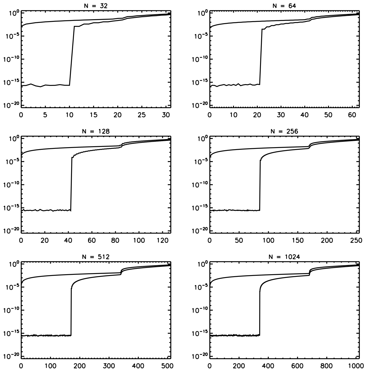
Fig. 6. Plots of \mathcal{E}_{j, \lfloor 2N/3 \rfloor}^{(1)} , and \mathcal{E}_{j, \lfloor 2N/3 \rfloor}^{(2)} for the cosine transform of a sine function for N \in \{32, 64, 128, 256, 512, 1024\} and j \leq N . In each plot, the top line shows \mathcal{E}_{j, \lfloor 2N/3 \rfloor}^{(1)} and the bottom line shows \mathcal{E}_{j, \lfloor 2N/3 \rfloor}^{(2)} . For clarity, the ratios, \mathcal{E}_{j, \lfloor 2N/3 \rfloor}^{(2,1)} , are not shown.
