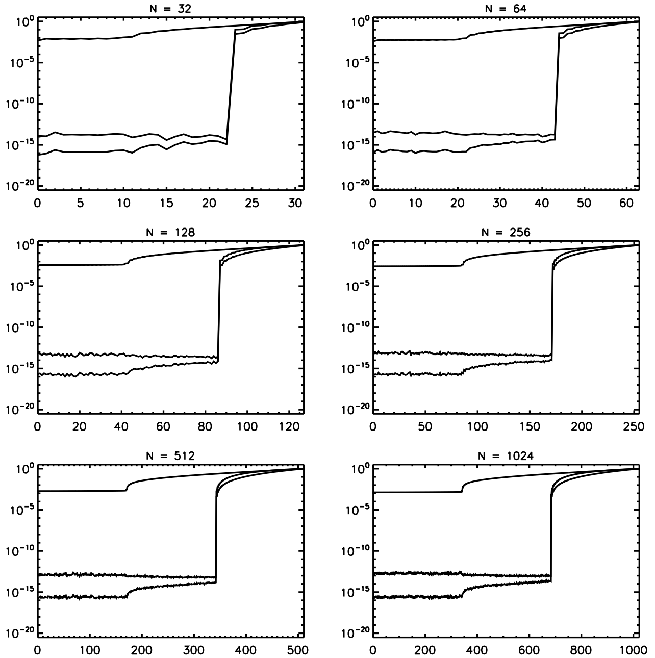
Fig. 1. Plots of \mathcal{E}_{j,[N/3]}^{(1)} , \mathcal{E}_{j,[N/3]}^{(2)} , and \mathcal{E}_{j,[N/3]}^{(2,1)} for the sine transform of a cosine function for N \in \{32, 64, 128, 256, 512, 1024\} and j \leq N . In each plot, the top line shows \mathcal{E}_{j,[N/3]}^{(1)} , the bottom line shows \mathcal{E}_{j,[N/3]}^{(2)} and the intermediate line shows the ratios, \mathcal{E}_{j,[N/3]}^{(2,1)} .
