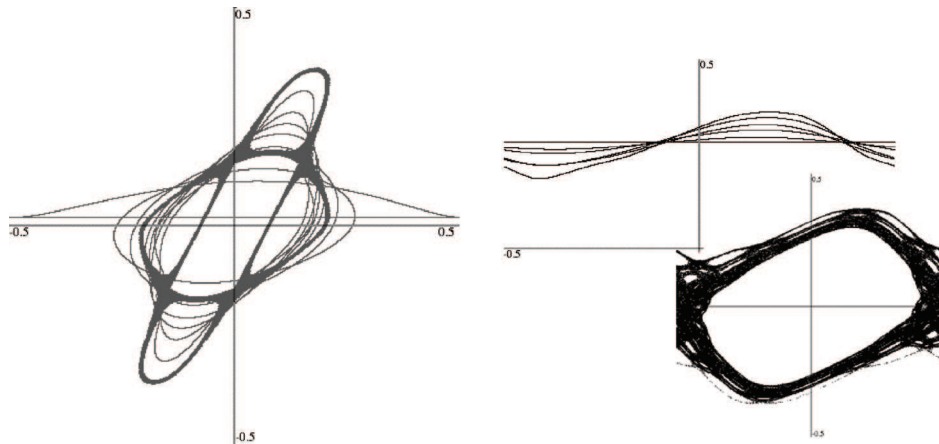
Figure 6. Overlay showing the evolution of two orbits beginning at k = 0 as k is incremented. In the left pane, an initial circle y \approx 0.02 evolves to the chaotic trajectory near a period-4 saddle when k = 2.25 . In the right pane, the initial circle at y \approx 0.3 evolves to chaotic orbit shown in the inset at k = 0.85 .
