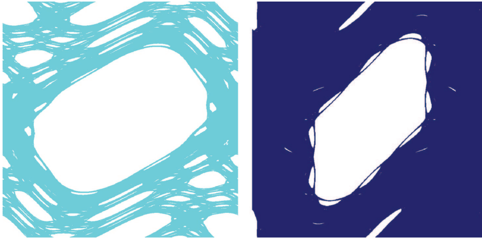
Figure 3. Chaotic orbits appear to densely cover a fat fractal like this set generated by iteration of a single initial condition for k = 1.0 (left pane) and k = 2.0 (right pane).
