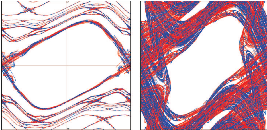
Figure 7. Stable and unstable manifolds for the standard map at k = 1.0 (left pane) and k = 2.0 (right pane). The left pane shows manifolds for the orbits (1, 2) , (2, 5) , (3, 8) , (1, 3) , (2, 7) , (0, 1) , (-2, 7) , (-1, 3) , (-3, 8) , (-2, 5) , (-1, 2) . The right pane shows only the manifolds for (0, 1) .
