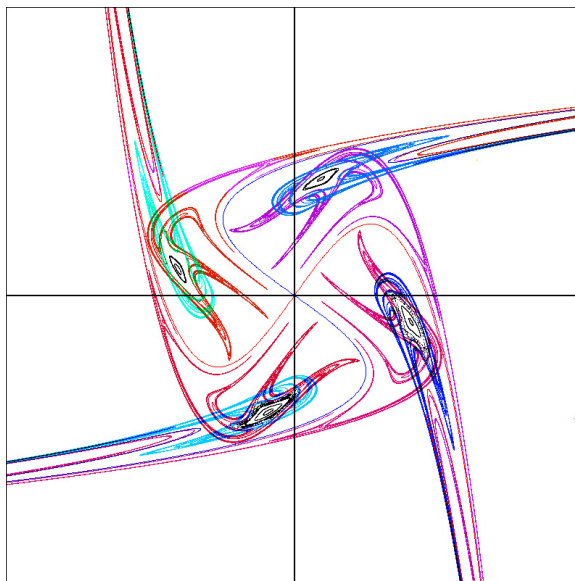
Figure 3: Some orbits of the map (43) for (b, \delta) = (1.4, 1.3) . There are elliptic fixed points at (0.27438, 1.2116) and hyperbolic points at (1.0010, 1.2794) , as well as the images of these points under \tau_\omega . The domain is the same as Fig. 2.
