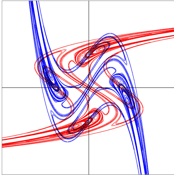
Figure 4: Some stable and unstable manifolds of the map (43) for (b, \delta) = (1.8, 1.3) . Here the elliptic points (e.g. at (0.23390, 1.3607) ) have undergone a period-doubling bifurcation. The domain is the same as Fig. 2.
