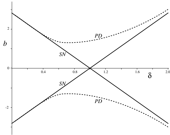
Figure 1: Bifurcation curves for the asymmetric fixed points of (43). The 8 asymmetric fixed points exist in the upper and lower quadrants of the cone. They undergo period-doubling bifurcations on the dashed curves.
