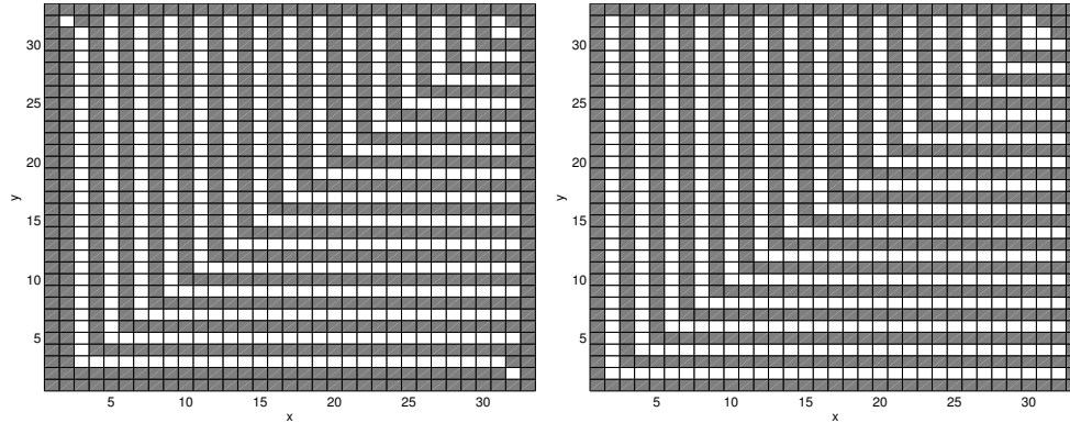
Figure 2. Coarse grids chosen for the non-grid-aligned anisotropic problem with 2 iterations of Jacobi (left) and Jacobi-preconditioned CG (right)
