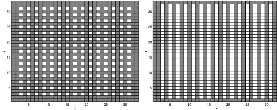
Figure 1. For the isotropic Poisson problem, the same coarse grid (shown at left) is chosen using the measure approximated by 2 iterations of Jacobi or Jacobi-preconditioned CG. The grid at left is also chosen for the diagonally scaled Poisson problem, using the measure approximated by two iterations of Jacobi or Jacobi-preconditioned CG. At right is the coarse grid chosen for the grid-aligned anisotropic problem, using either two iterations of Jacobi or Jacobi-preconditioned CG to approximate the strength of connection measure.
