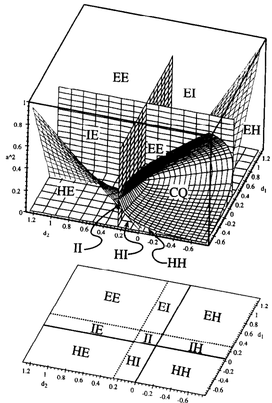
Fig. 1. Stability of minimizing orbit for a 4D map in the space of the three essential parameters d_1, d_2 and the square of the antisymmetry of the twist a^2 .
